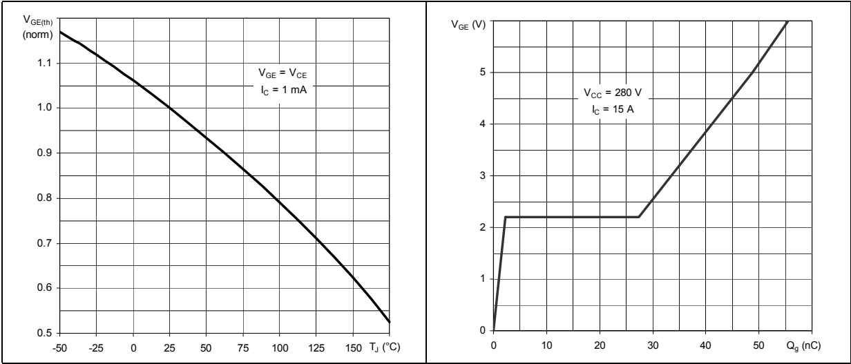
Figure 10. Normalized gate threshold voltage vs temperature Figure 11. Gate charge
